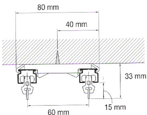
Support double
